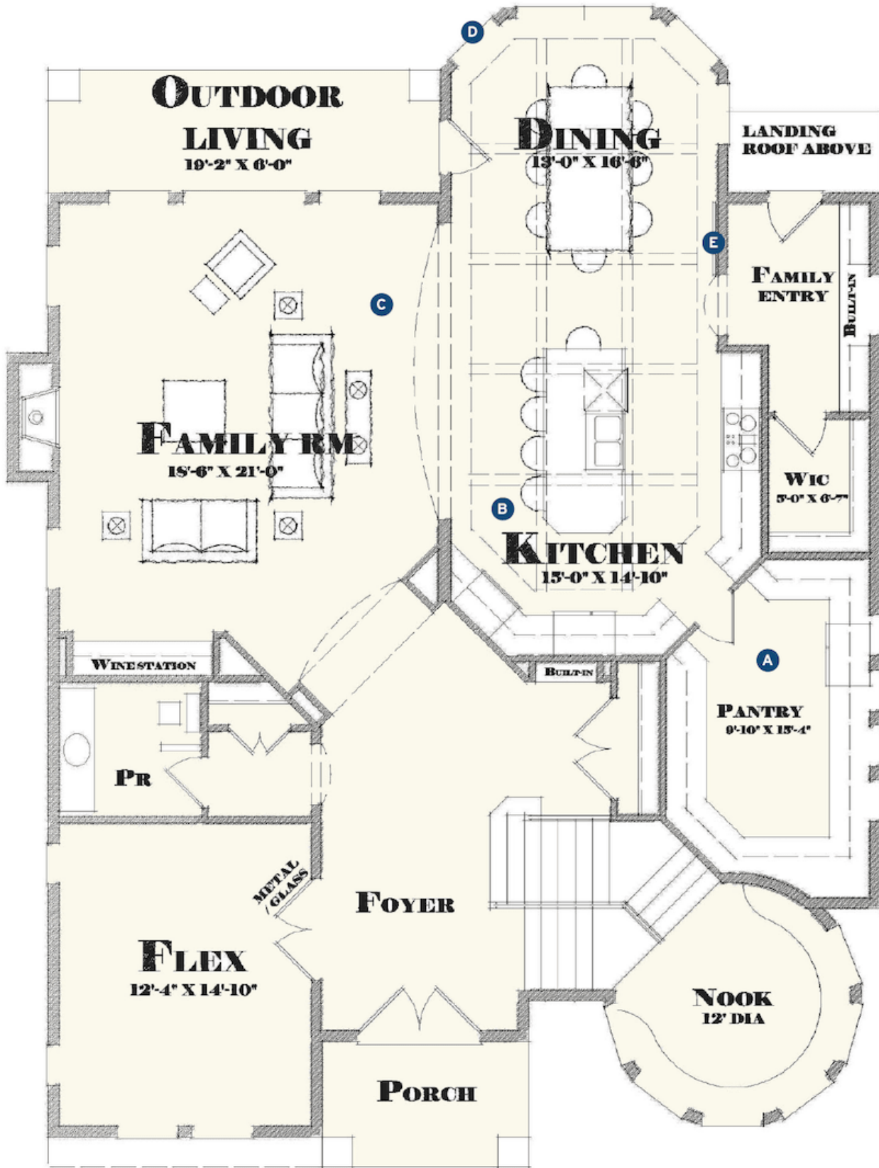
FIRST FLOOR
